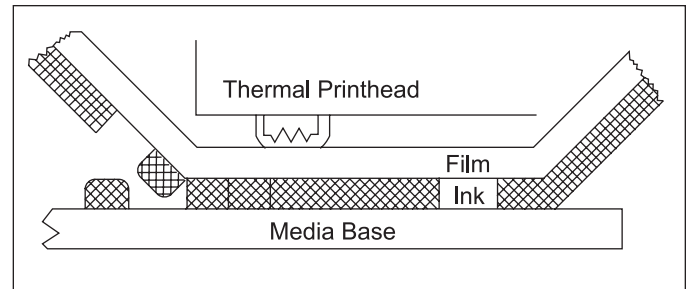
Figure 6. Thermal Transfer Printing
